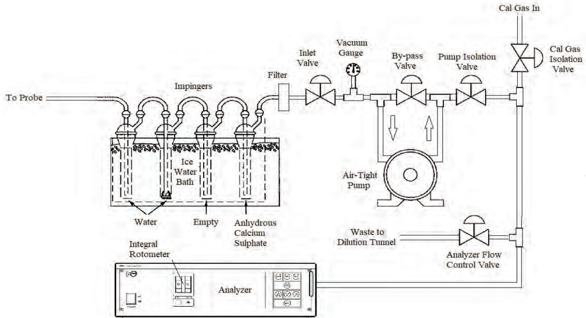
Figure 15 - Flue Gas Measurement System
